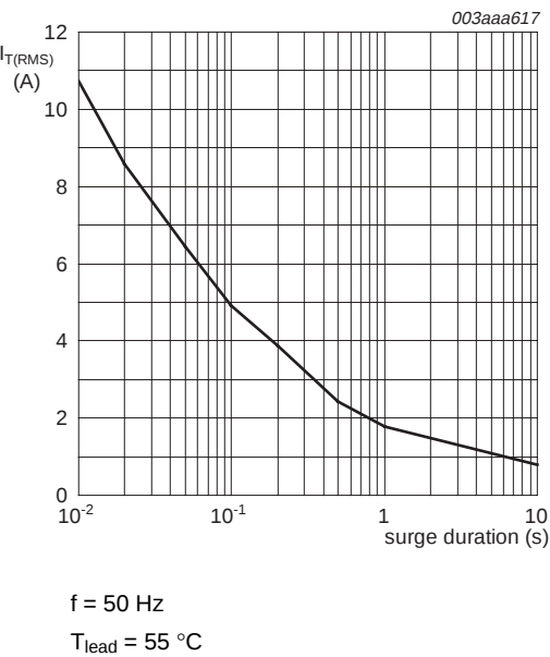
Fig 4. RMS on-state current as a function of surge duration; maximum values
